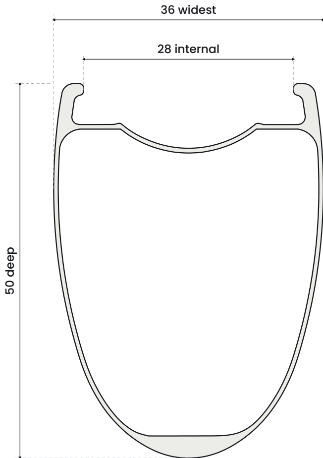
Section at 2:1 when printed at 100% on A4. Figures in mm.
