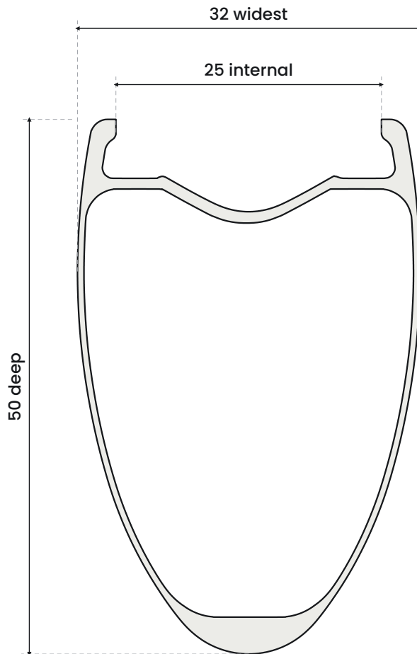
Section at 2:1 when printed at 100% on A4. Figures in mm.
